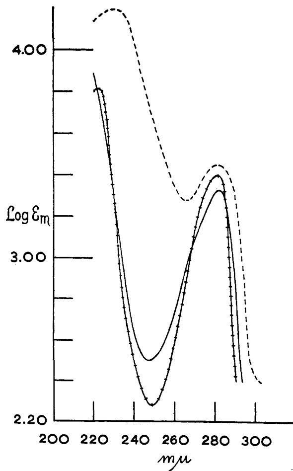
Fig. 1.—Ultraviolet absorption spectra (in 95% ethanol): -----, 3-hydroxy-17-acetyl-1,3,5,16-estratetraene (VIIa); + + + +, 3-hydroxy-17-acetyl-1,3,5-estratriene (IXa); —————, 3-hydroxy-16-methoxy-17-acetyl-1,3,5-estratriene (VIII).
